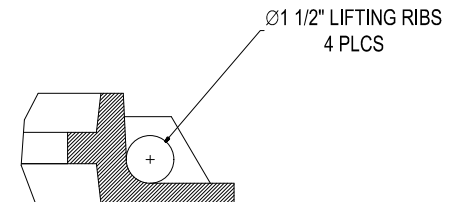
LIFTING RIB
