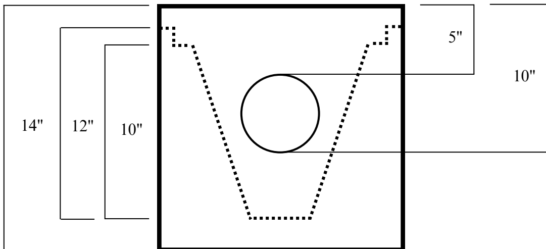
Side View
